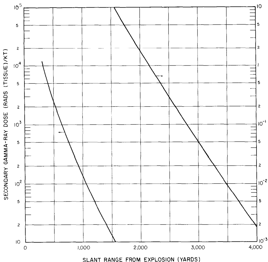
Figure 8.127b. Air-secondary gamma-ray component of the initial nuclear radiation dose per kiloton yield as a function of slant range from thermonuclear weapon air bursts, based on 0.9 normal sea-level air density.
