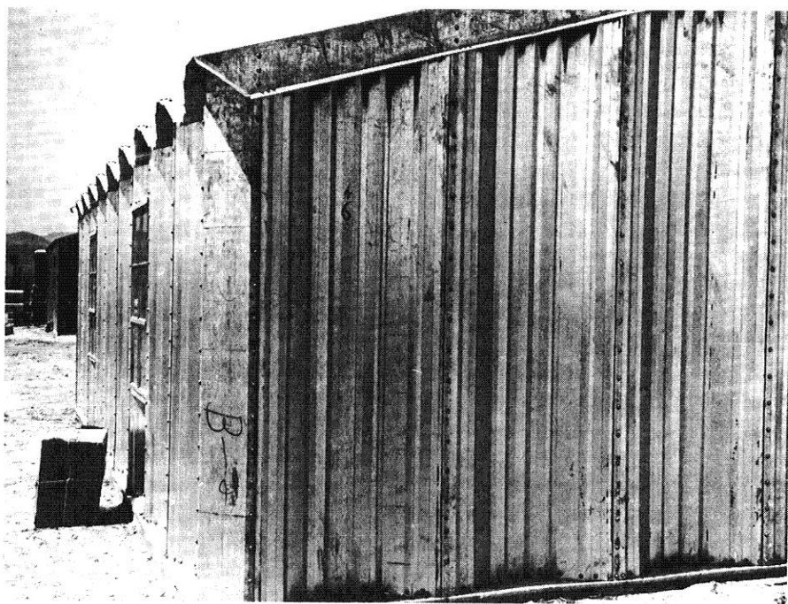
Figure 5.43. Self-framing corrugated steel panel building before a nuclear explosion, Nevada Test Site.
