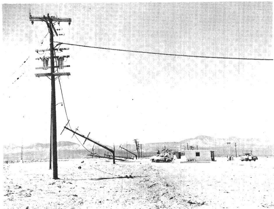
Figure 5.104. Collapse of utility poles on line (5 psi peak overpressure, 0.6 psi dynamic pressure from 30-kiloton explosion), Nevada Test Site.
