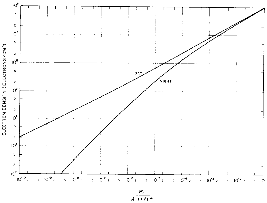
Figure 10.159a. Electron density at 40-mile altitude due to beta particles (for debris above 40 miles).
