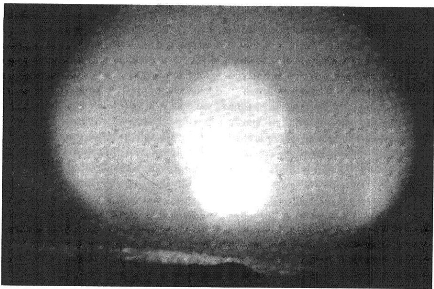
Figure 2.56. Fireball and red luminous spherical wave formed after the TEAK high-altitude shot. (The photograph was taken from Hawaii, 780 miles from the explosion.)
