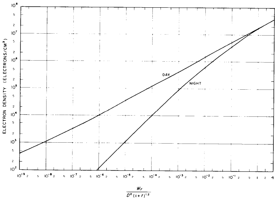
Figure 10.159b. Electron density at 40-mile altitude due to delayed gamma rays (for debris above 15 miles).
