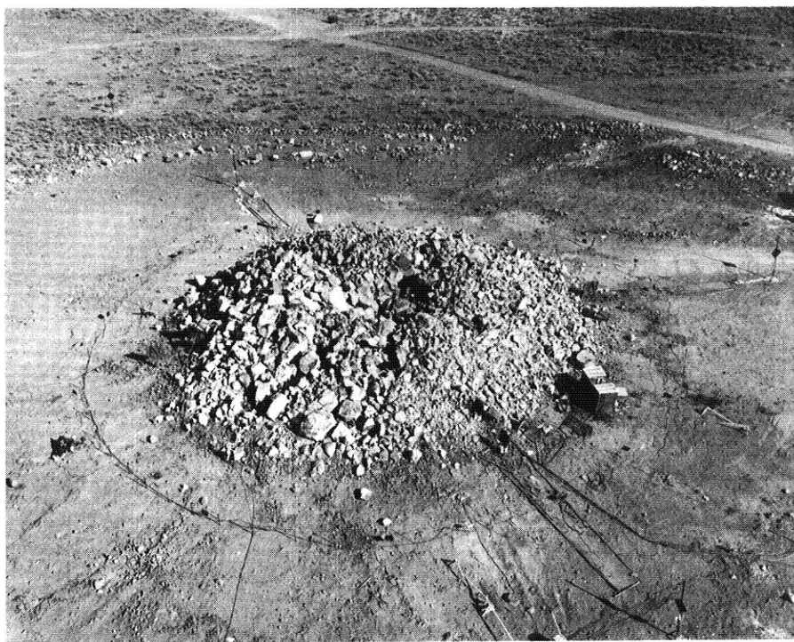
Figure 6.05. SULKY event; mound created by the bulking of rock material in a 0.087-kiloton nuclear detonation at a depth of 90 feet.
